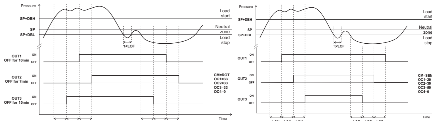
Fig.3 Control by sequential activation of outputs
