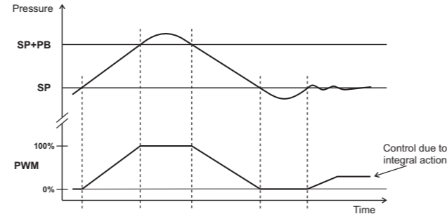
Fig.5 PWM output control
