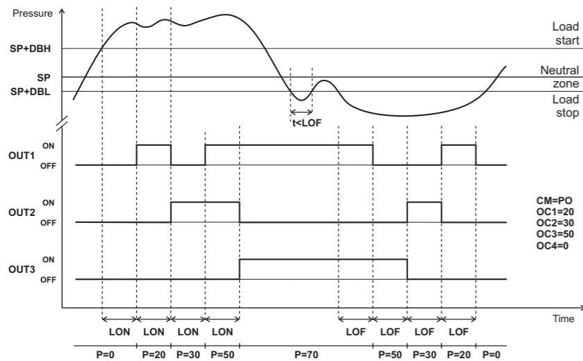
Fig.4 Control by optimisation of the available power
